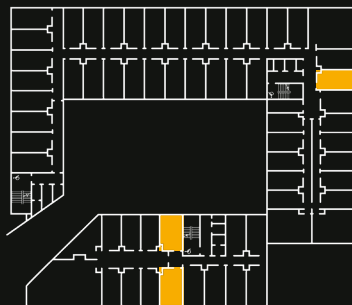
LEVEL 1-4 (BLK 4)
